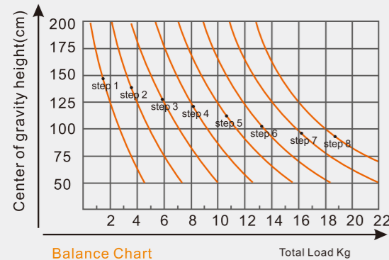
COUNTERBALANCE GRAPH
