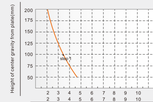
Balance Chart
