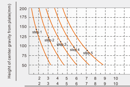
Balance Chart
