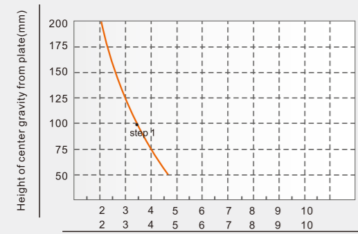
Balance Chart
